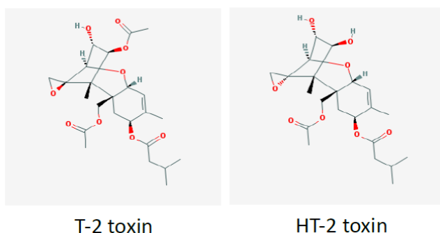
Figure 1. Chemical structures of T-2 and HT-2 (PubChem, 2025).
