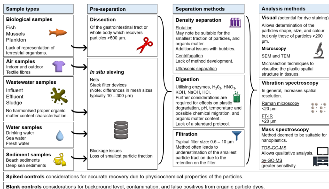
Figure 1. Provides an overview of the methodologies utilised in the separation and analysis of microplastics and nanoplastics in complex environmental
