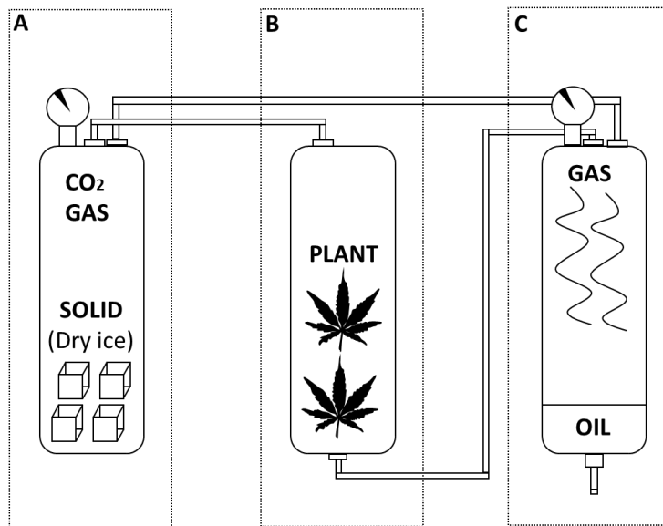
Figure 4. Supercritical fluid CO 2 extraction method A. solid dry pressurised CO 2 (commonly known as 'dry ice' B. dry plant material C. CO 2 -cannabinoid mixture is then pumped into a third chamber where it is kept at an even lower pressure and higher temperature so that the CO 2 gas rises to the top of the chamber while the oils containing chemicals and flavours from the plant material fall to the bottom to be collected for consumption.
